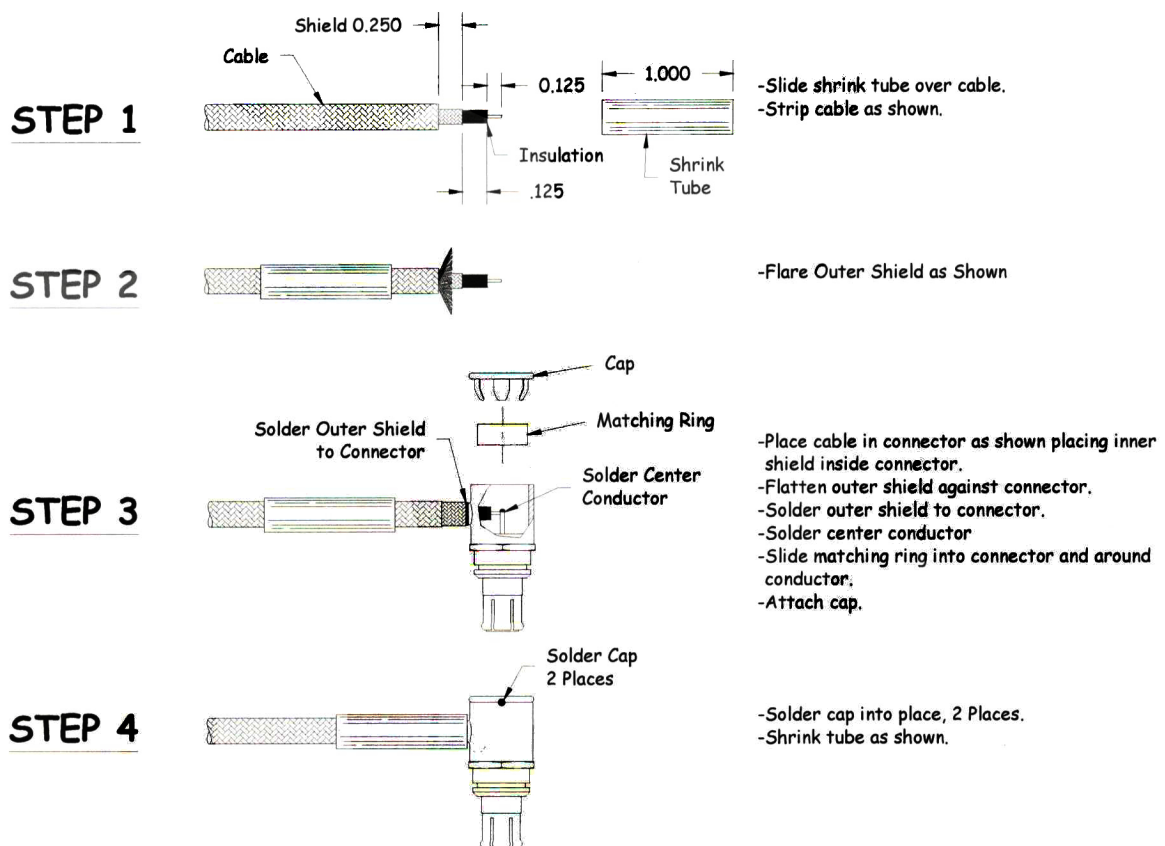
Figure 4 Coax Cable Assembly
