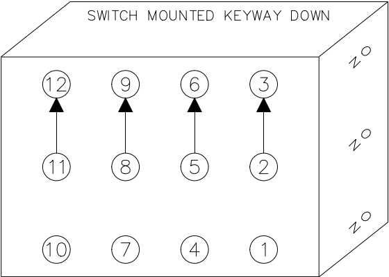
TOGGLE IN DOWN POSITION (AT KEYWAY)
