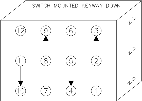
TOGGLE IN CENTER POSITION
