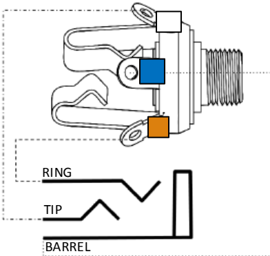
Headphone
